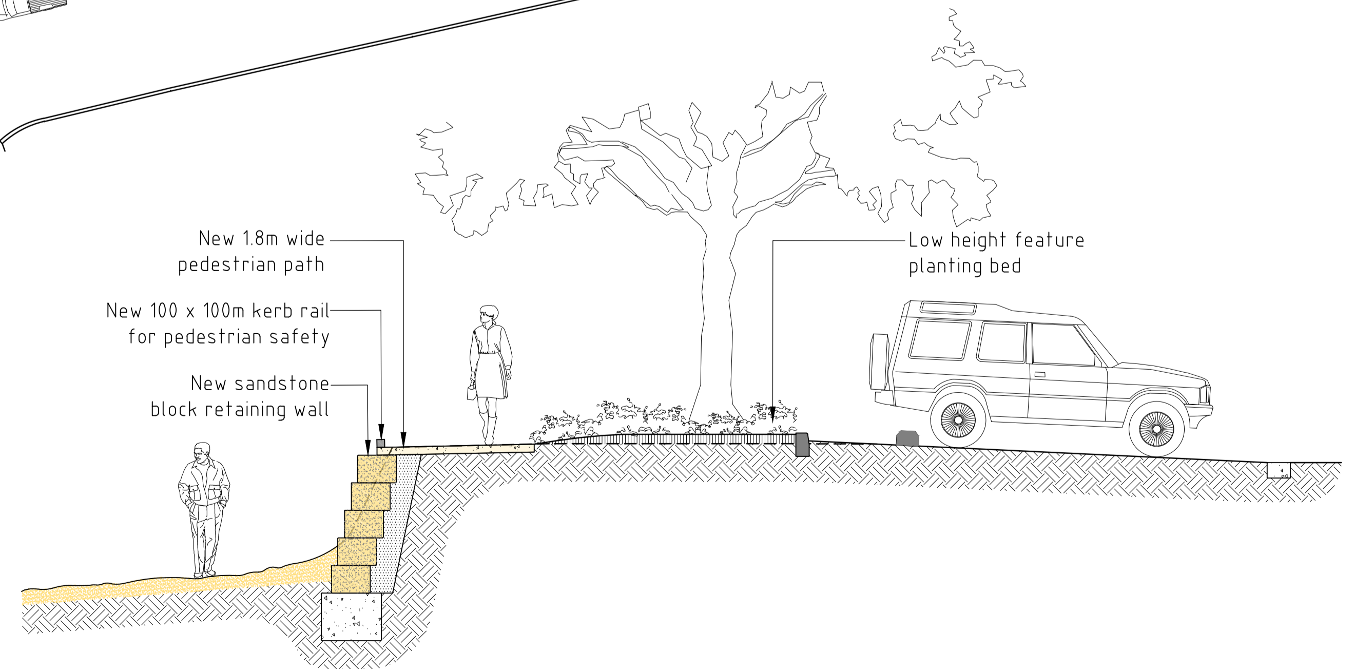
AA SHARED PATH CROSS SECTION Scale 1:50 @ A1
